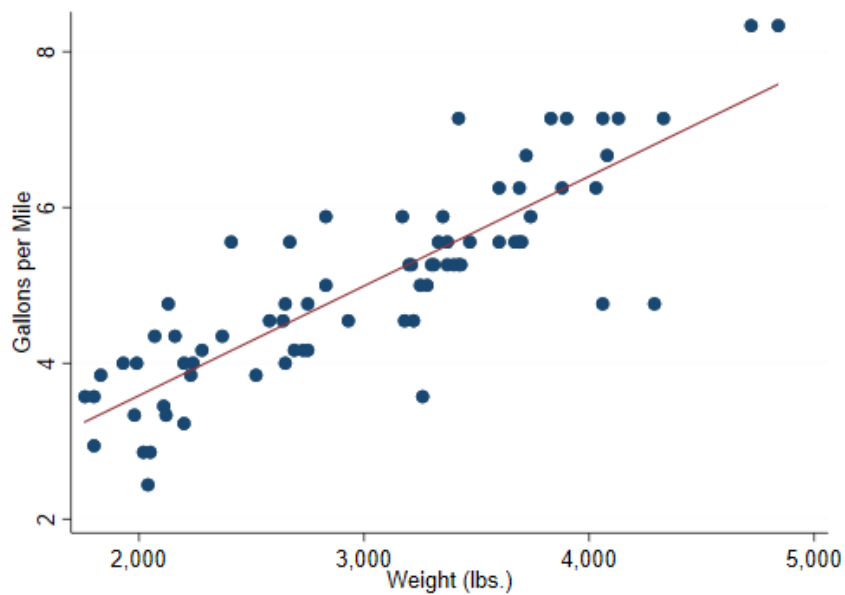
Figure 1: Fuel Efficiency
